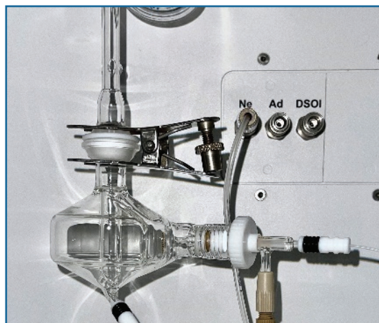
Figure 4. Slurry nebulizer
