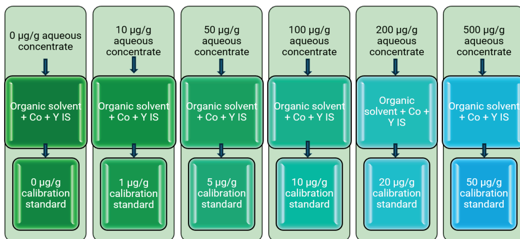
Figure 2. Calibration standard preparation using 10x aqueous metals concentrates
