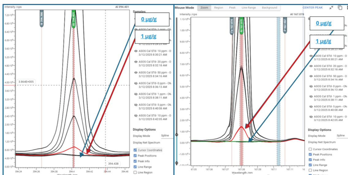
Figure 6. 0 \mu\text{g/g} and 1 \mu\text{g/g} standards for Al 394.401 nm and Al 167.078nm.
